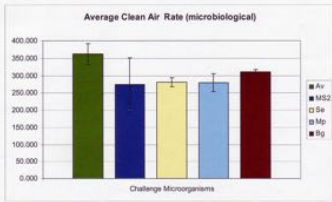
Figure 8. CAR m values for organisms tested
